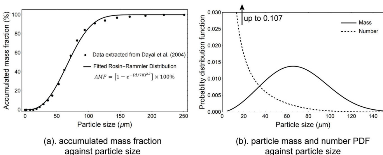
Fig 3. Spray drug particle size distribution used in the CFD simulation. (a) Measured data from Dayal et al. [30] showing cumulative mass fraction, fitted using Rosin-Rammler Distribution. (b). The corresponding mass and number probability distribution function over particle size. The range of particle size released was 1 – 150 μm.
