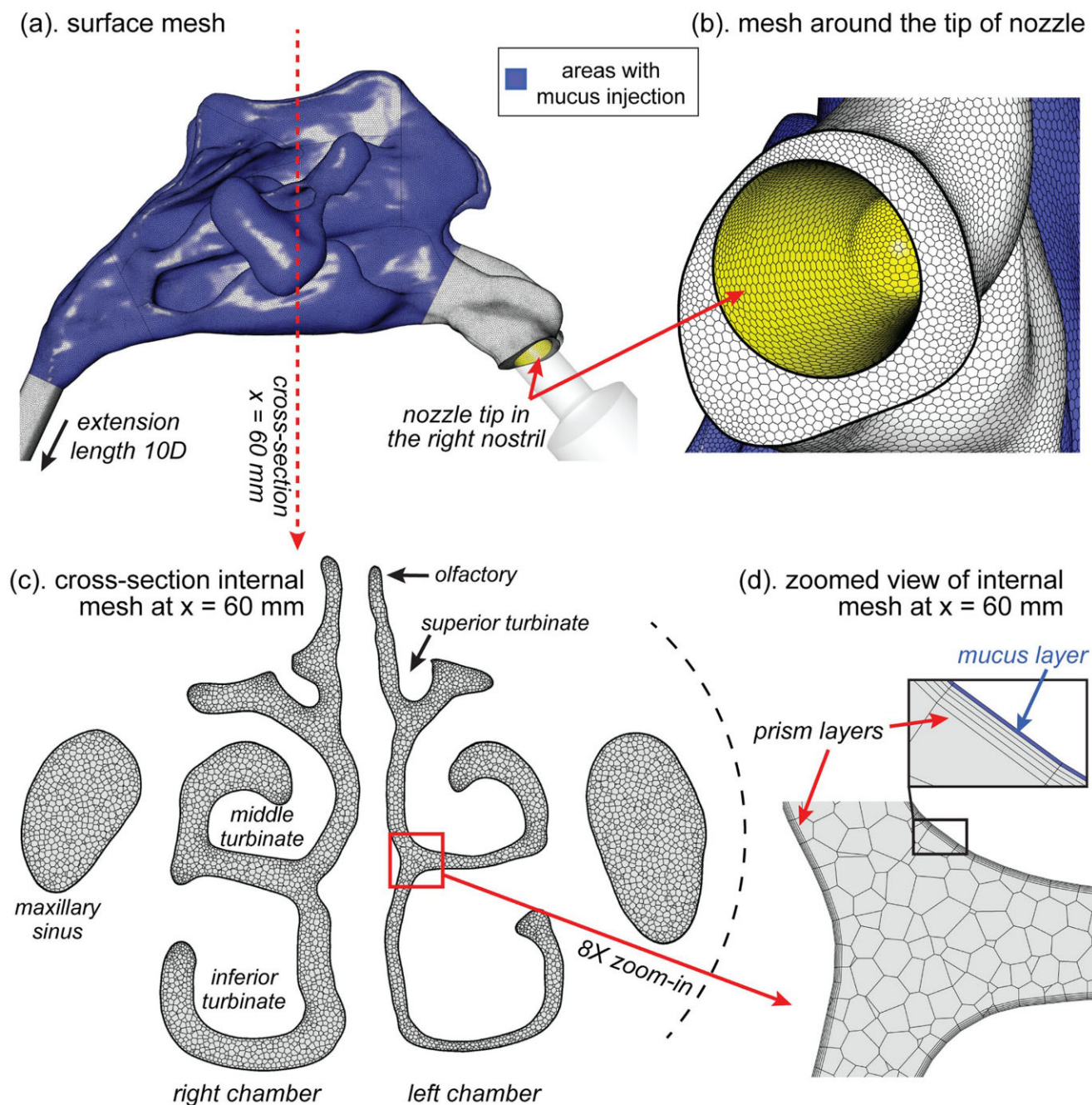
Fig 12. The CFD nasal cavity model contained polyhedral mesh elements. (a) Surface mesh on the vestibule, the nasal cavity and the outlet extension. All surface areas were covered with a 10\ \mu\text{m} thick mucus layer, but the source term for mucus injection was applied in the main nasal cavity only (coloured in blue). An extension from the nasopharynx exit was extruded with a length of 10 times its diameter to ensure fully developed flow at the outlet. (b) Refined surface mesh around the nozzle tip. (c) Cross section slice located at 60 mm away from the tip of nose showing the internal mesh. It also shows major anatomical regions including superior/middle/inferior nasal passages, superior/middle/inferior turbinates, olfactory regions and maxillary sinuses. (d) 8X zoomed view of the internal mesh containing polyhedral cells, prism layers and thin mucus layer (coloured in blue).
