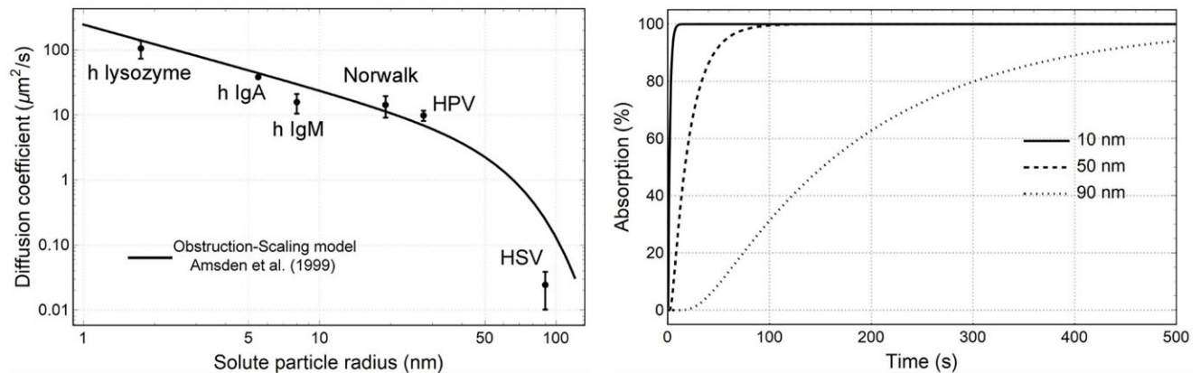
(a). Diffusion coefficient in mucus gel over solute radius
